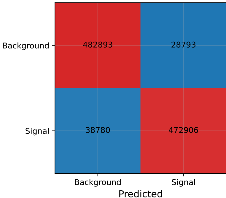
Confusion matrix (Test)
