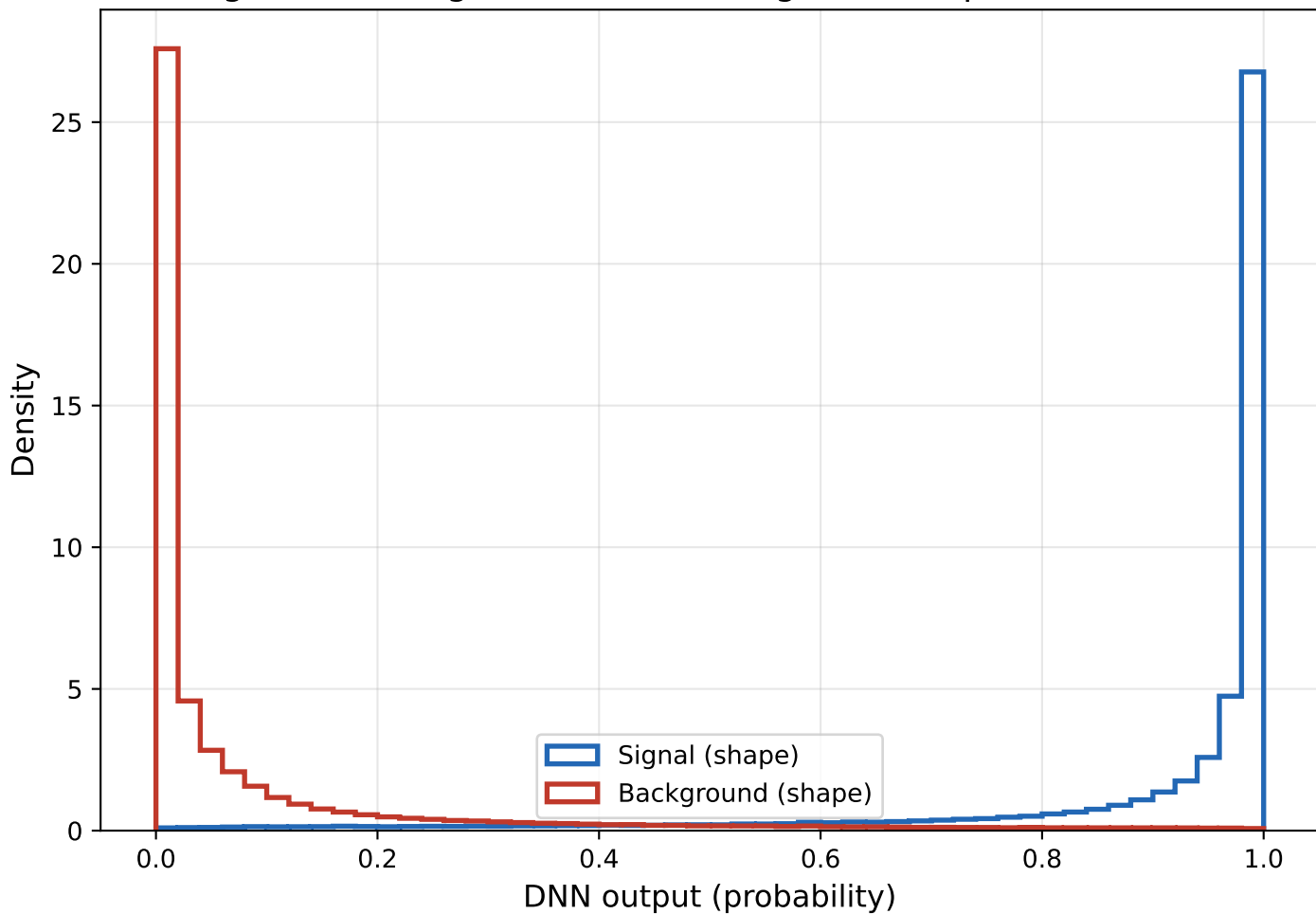
Signal vs Background -- Test (weighted, shape-normalized)
