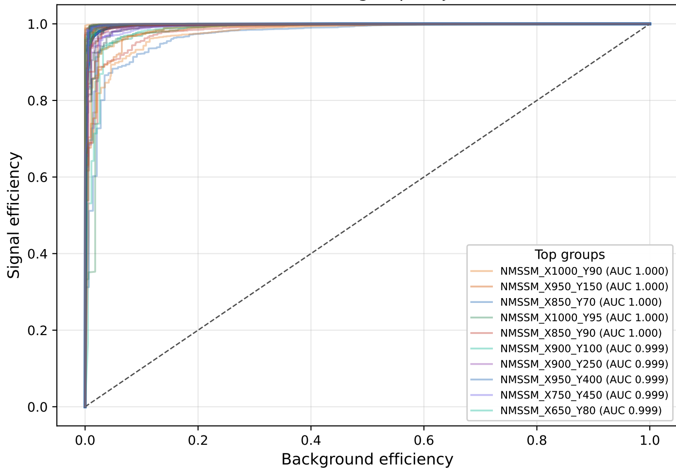
ROC -- Test (group-disjoint)
