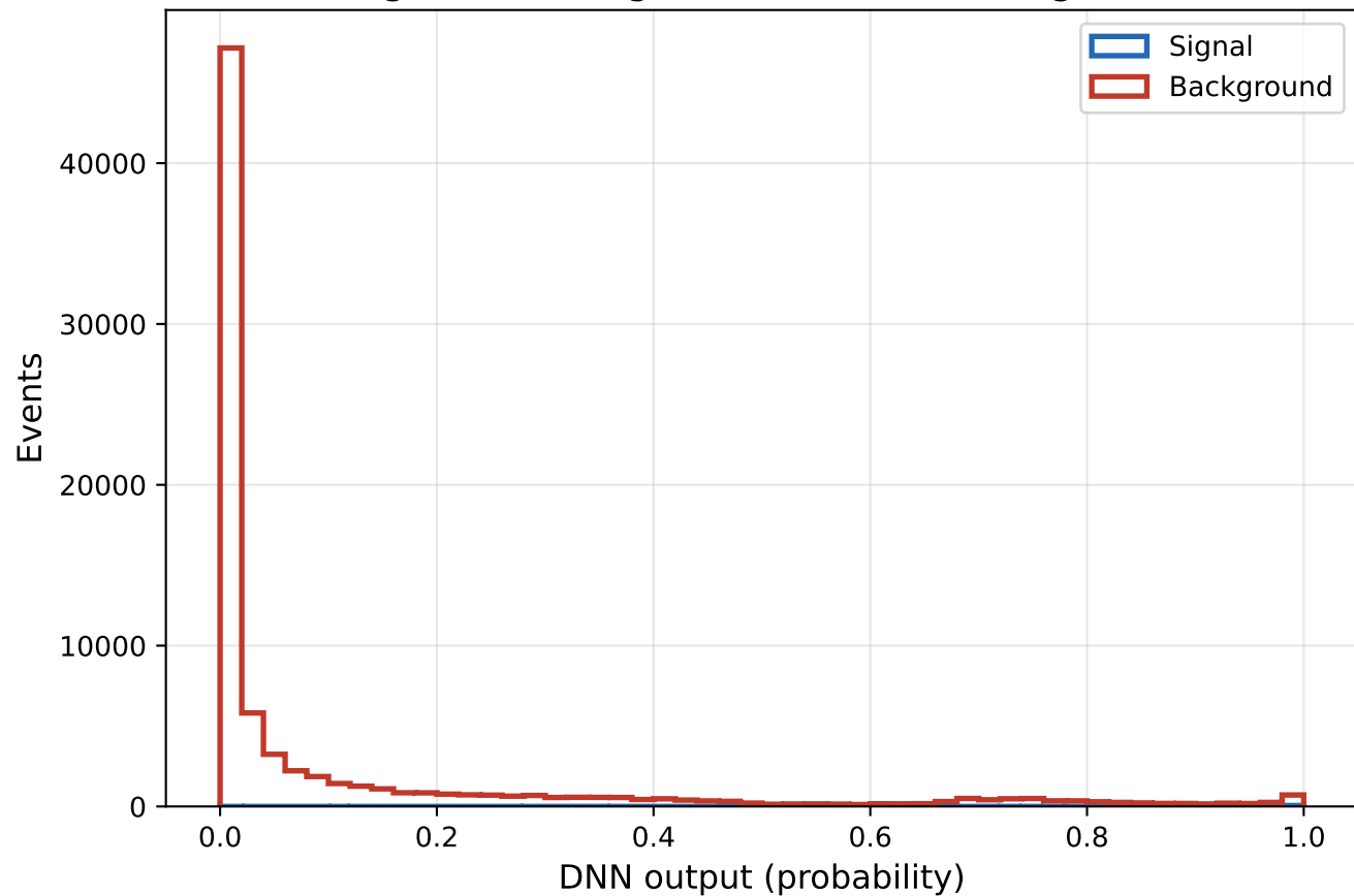
Signal vs Background -- Train (unweighted)
