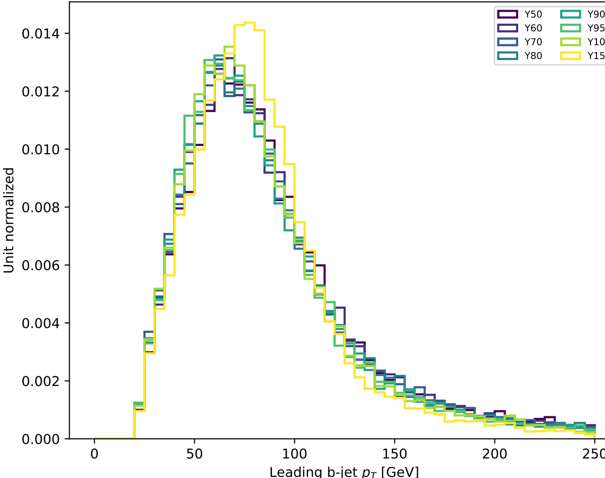
Lead b-jet p_T , X300
