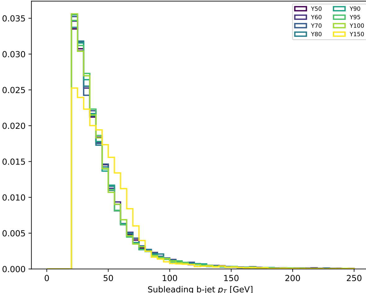
Sublead b-jet p_T , X300
