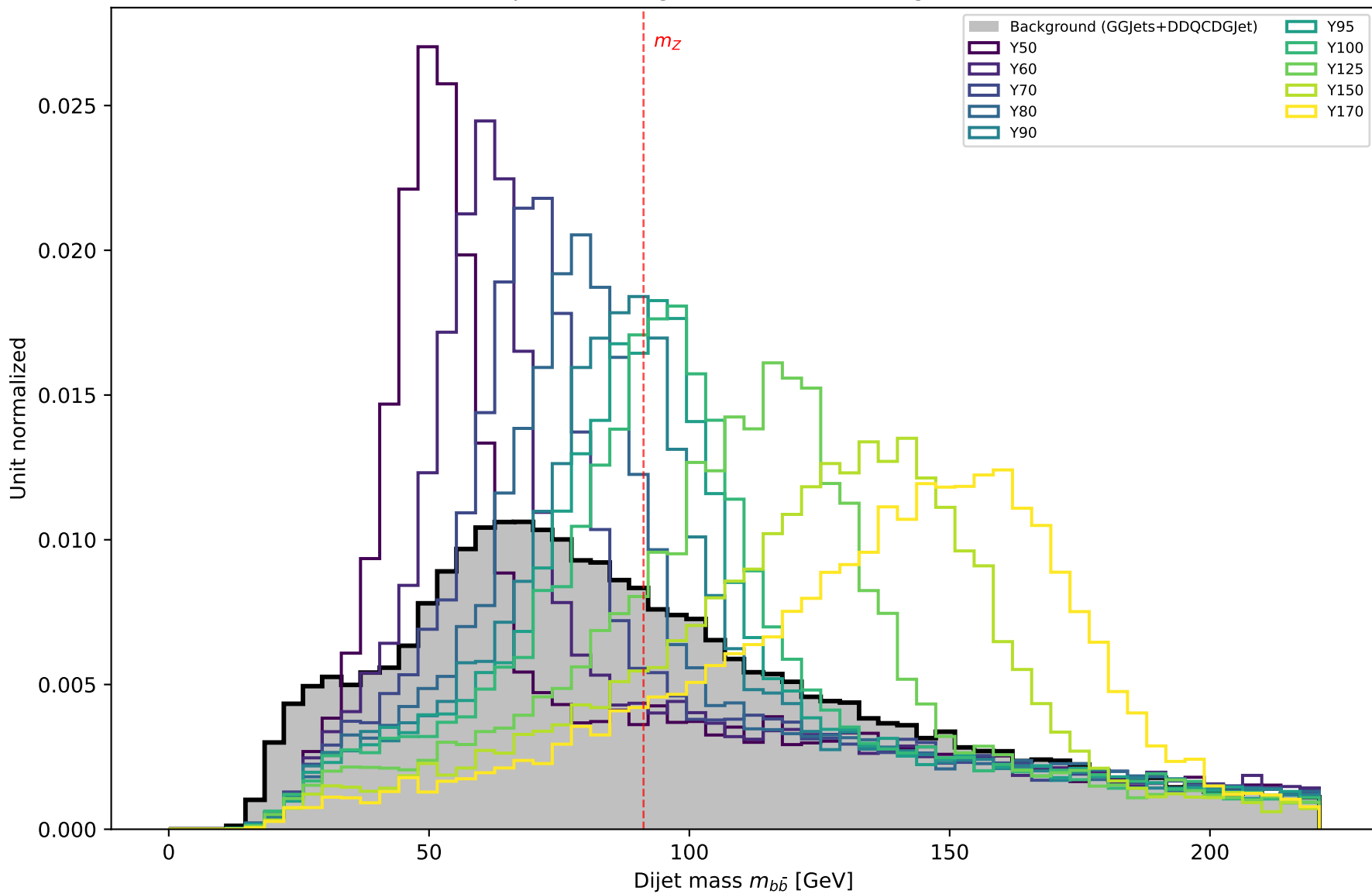
Dijet mass: signal (X300) vs. background
