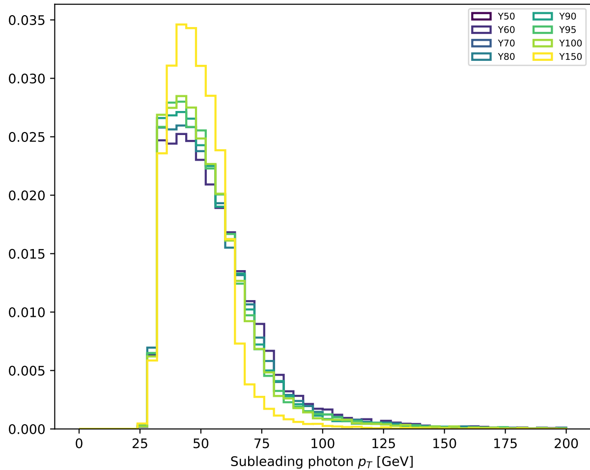
Sublead photon p_T , X300
