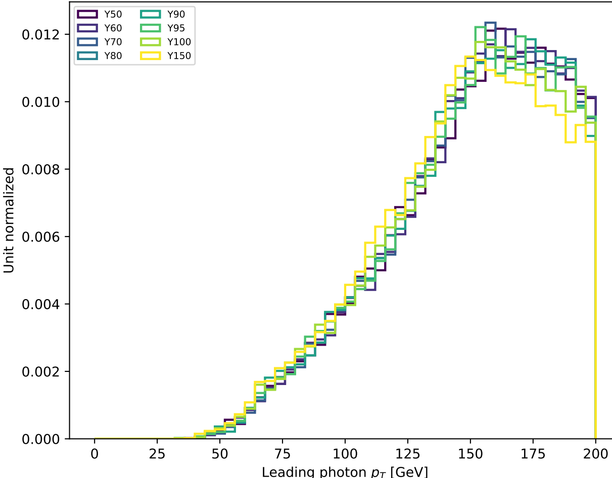
Lead photon p_T , X600
