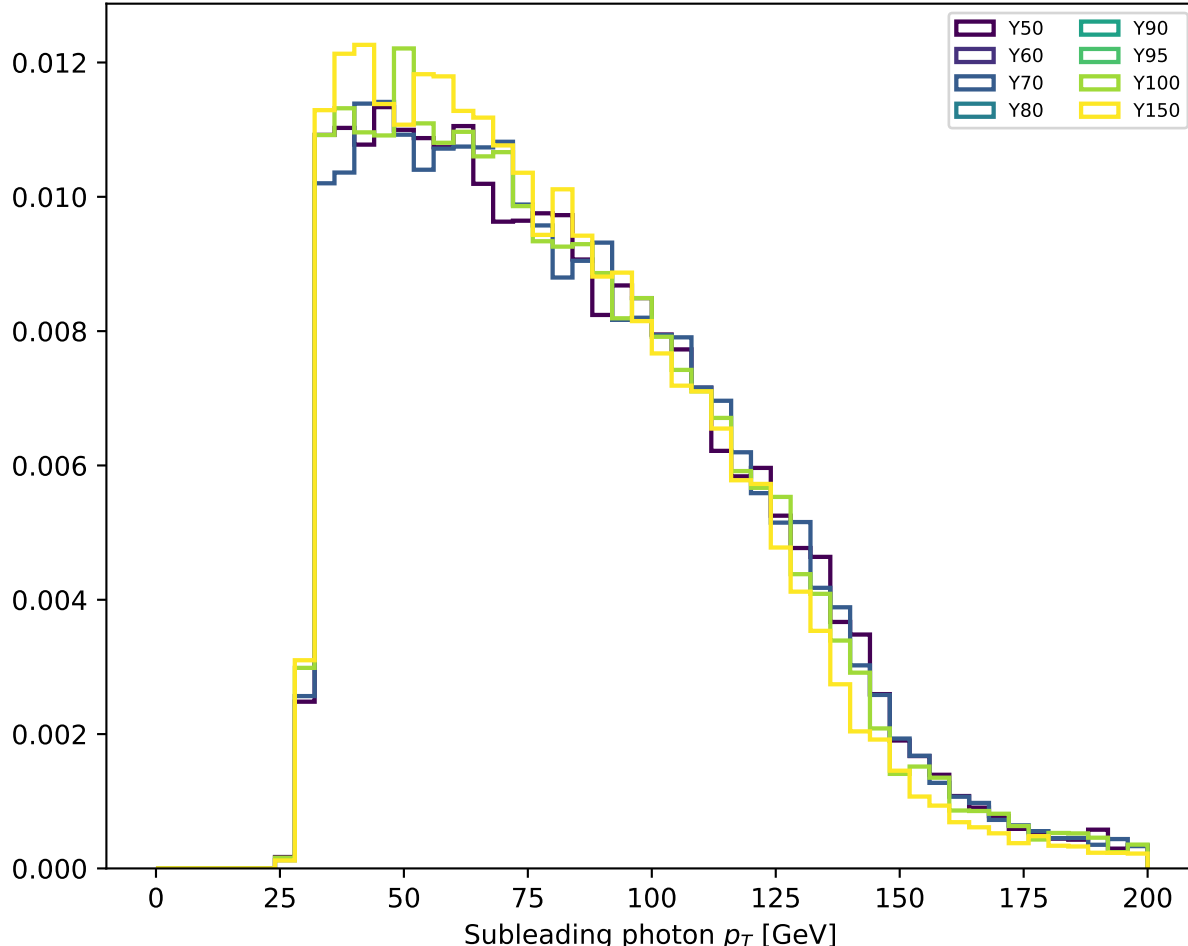
Sublead photon p_T , X600
