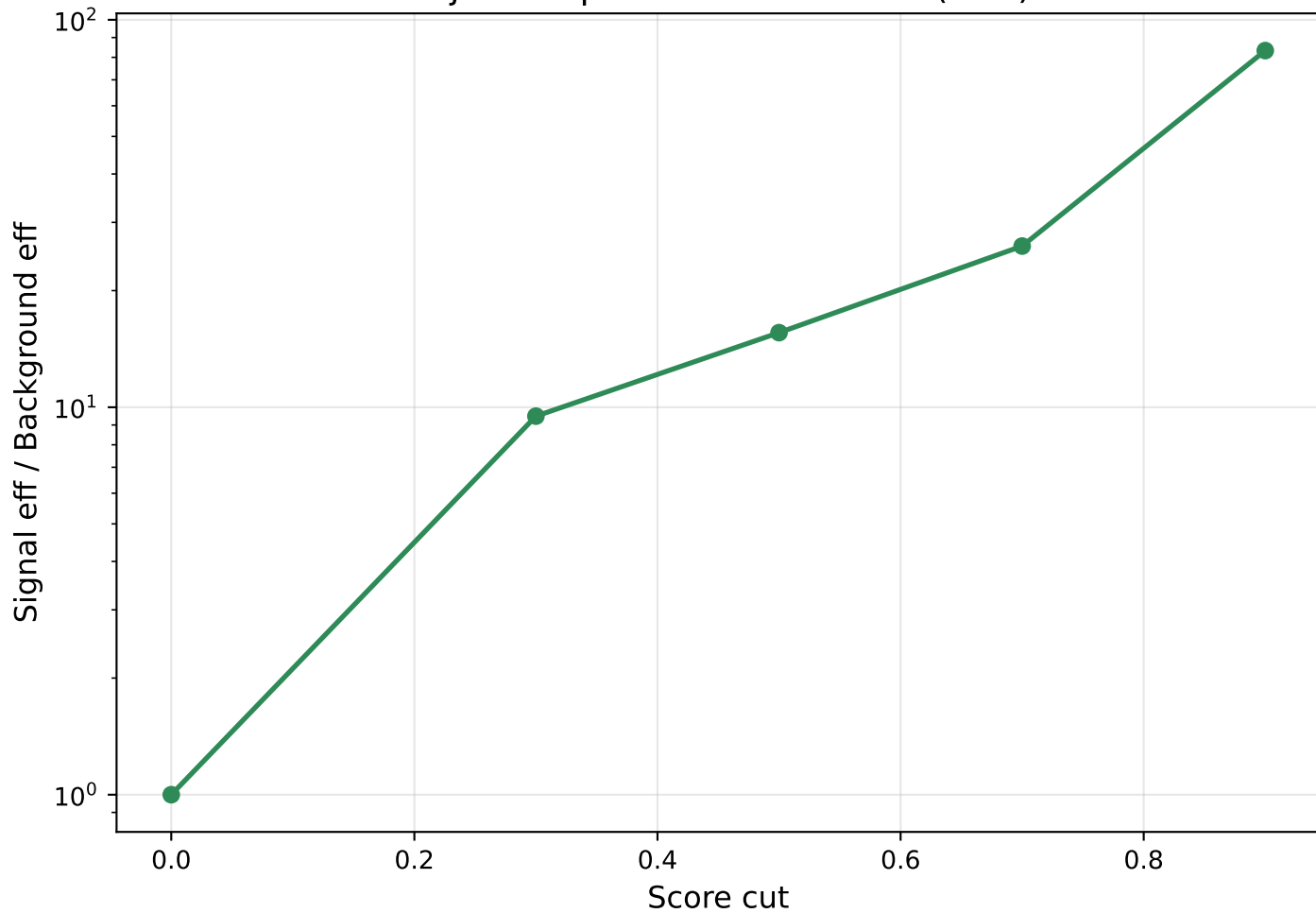
Rejection power vs. score cut (Test)
