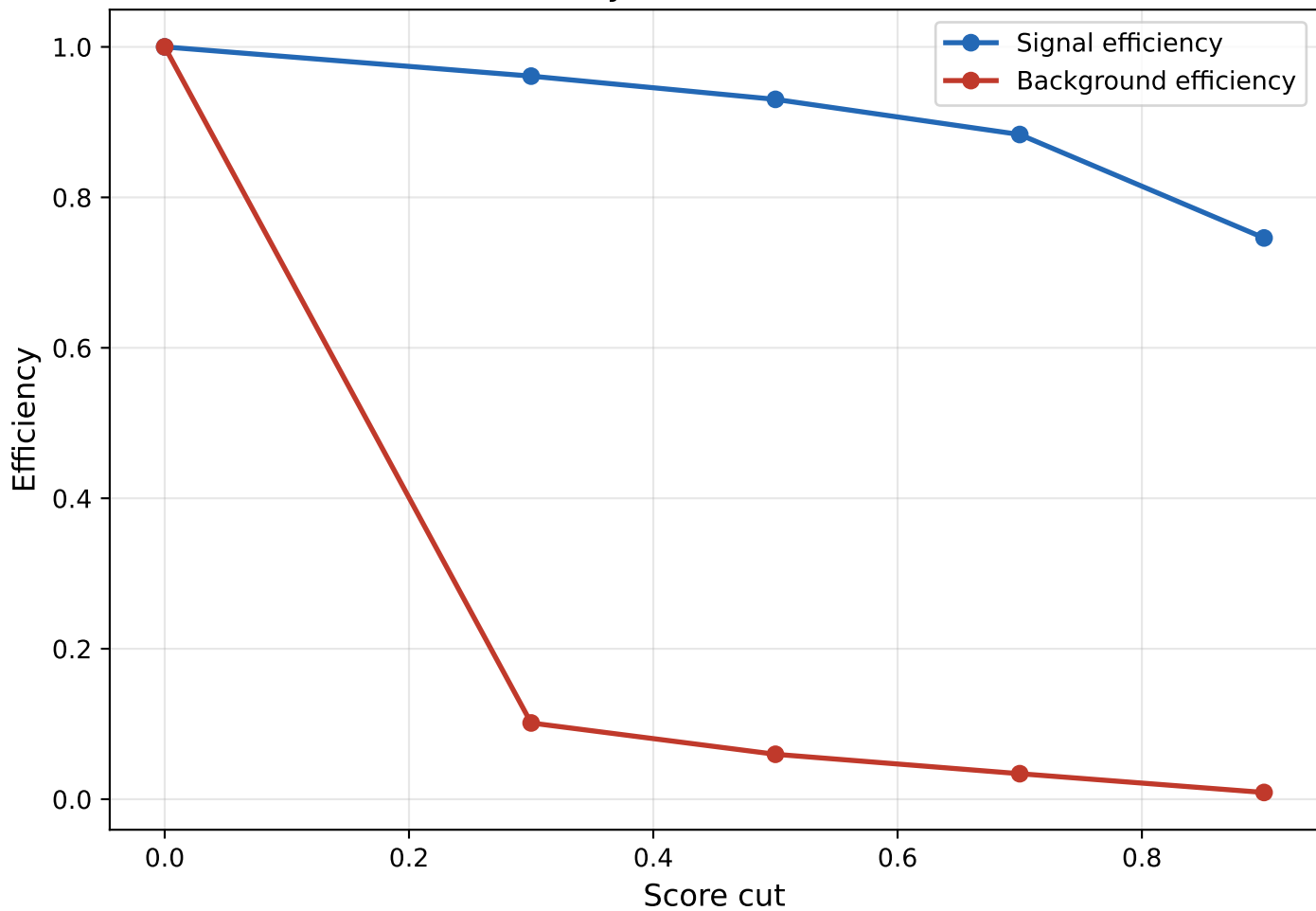
Efficiency vs. score cut (Test)
