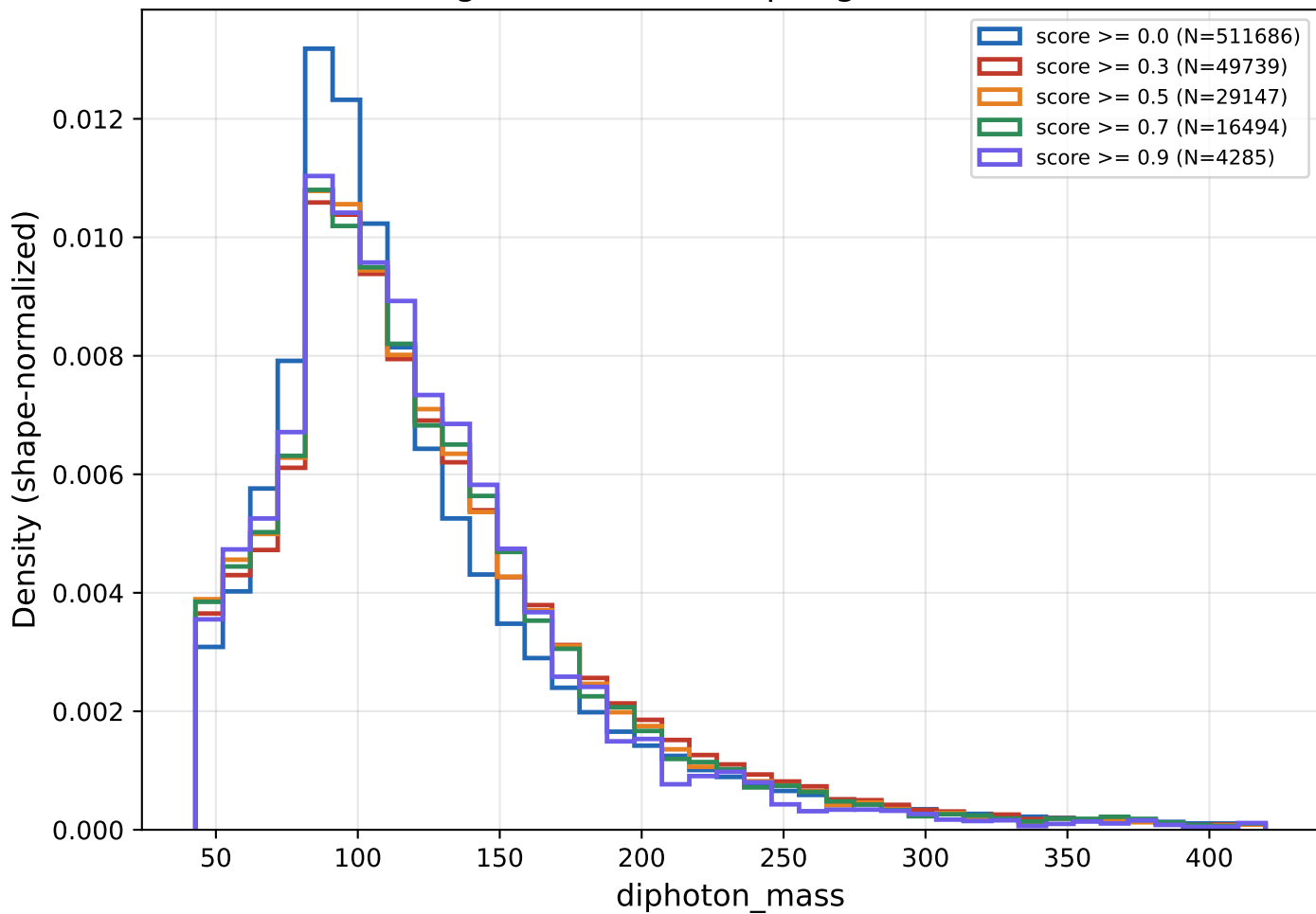
Background mass sculpting vs. score cut
