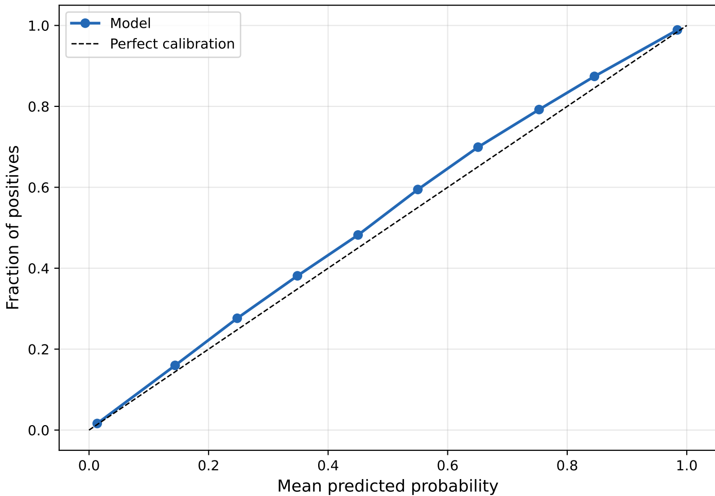
Calibration curve (Test)
