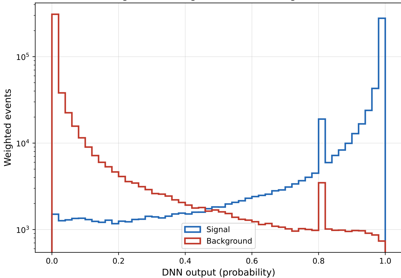
Signal vs Background -- Test (weighted)
