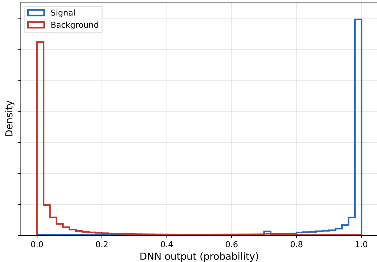
Signal vs Background -- Test (shape)
