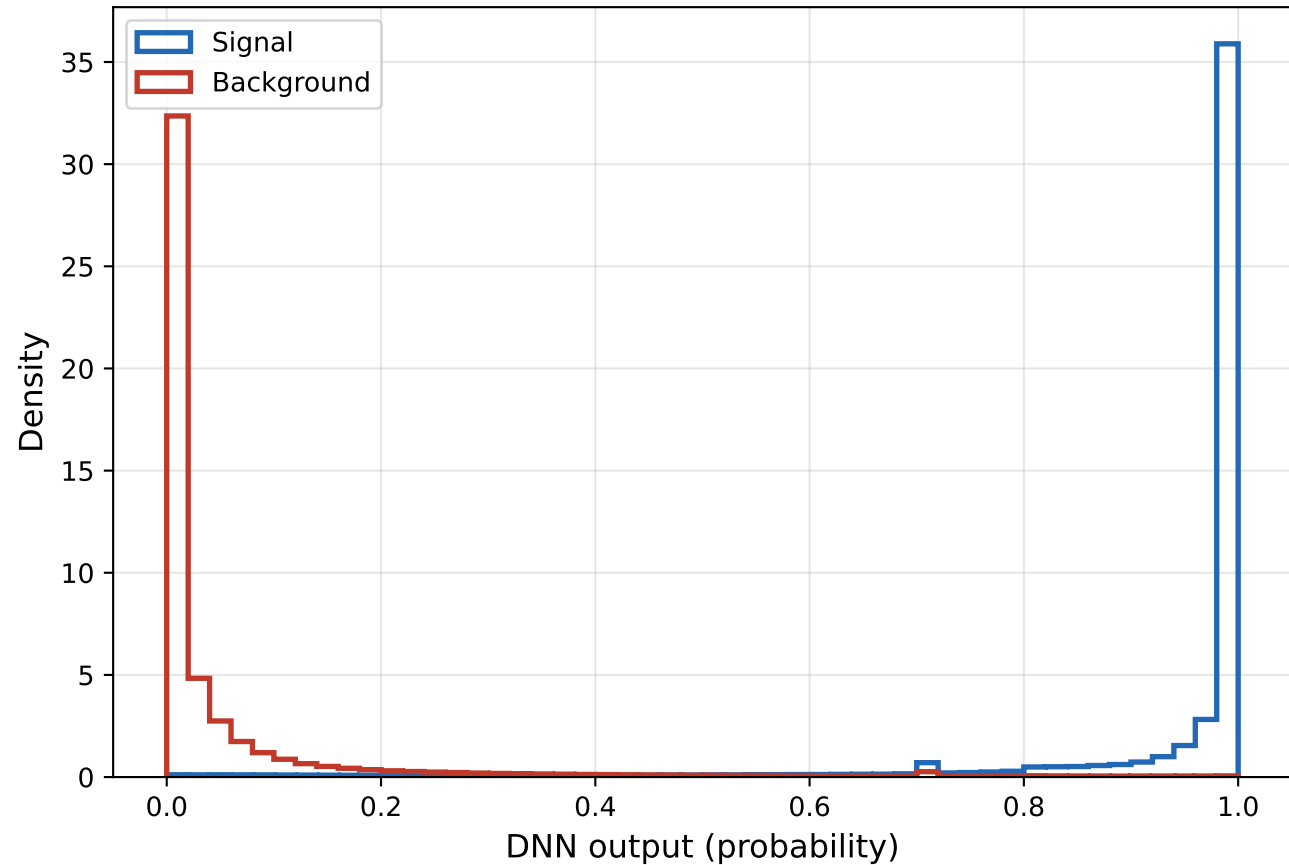
Signal vs Background -- Train (shape)
