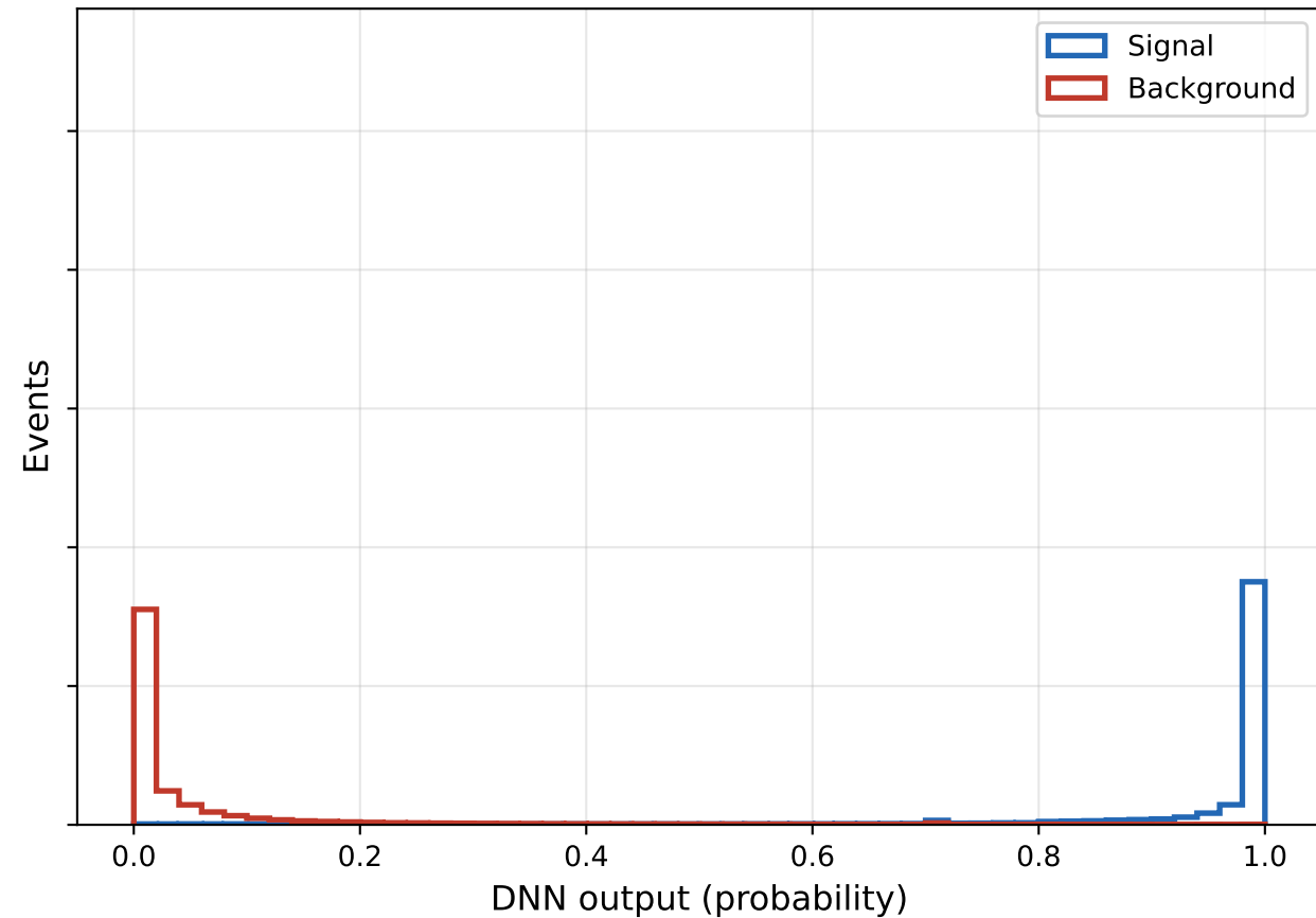
Signal vs Background -- Test (unweighted)
