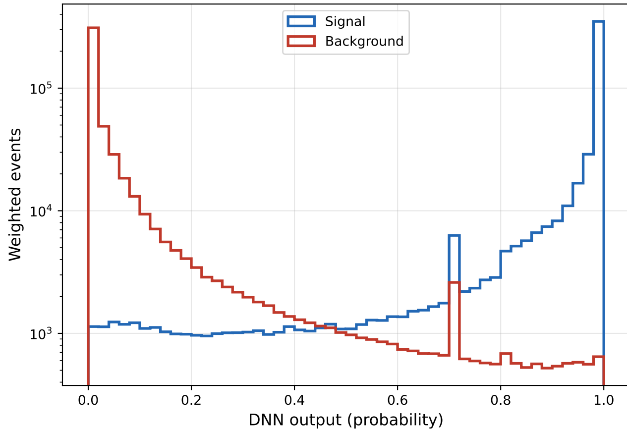
Signal vs Background -- Test (weighted)
