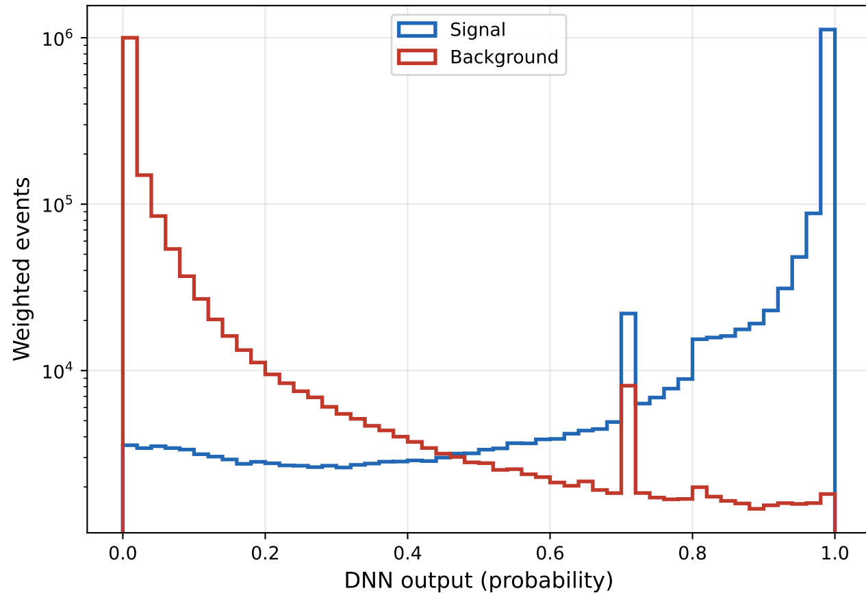
Signal vs Background -- Train (weighted)
