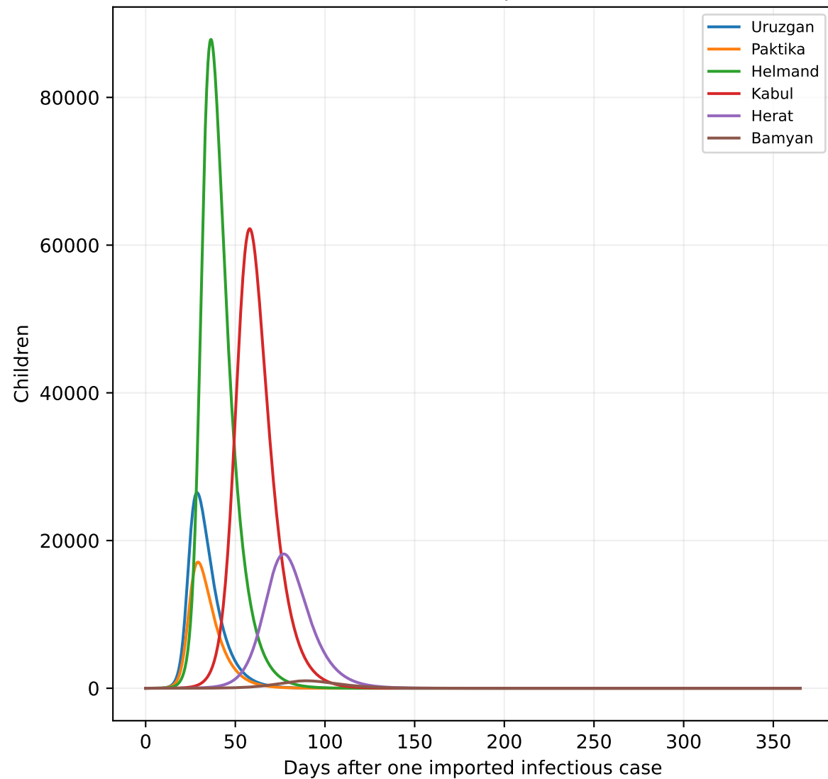
Infectious compartment
