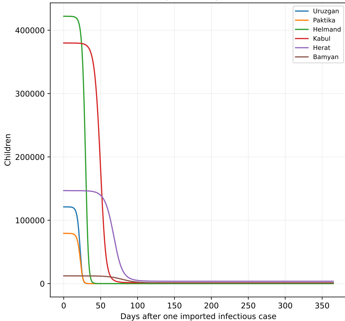
Susceptible compartment
