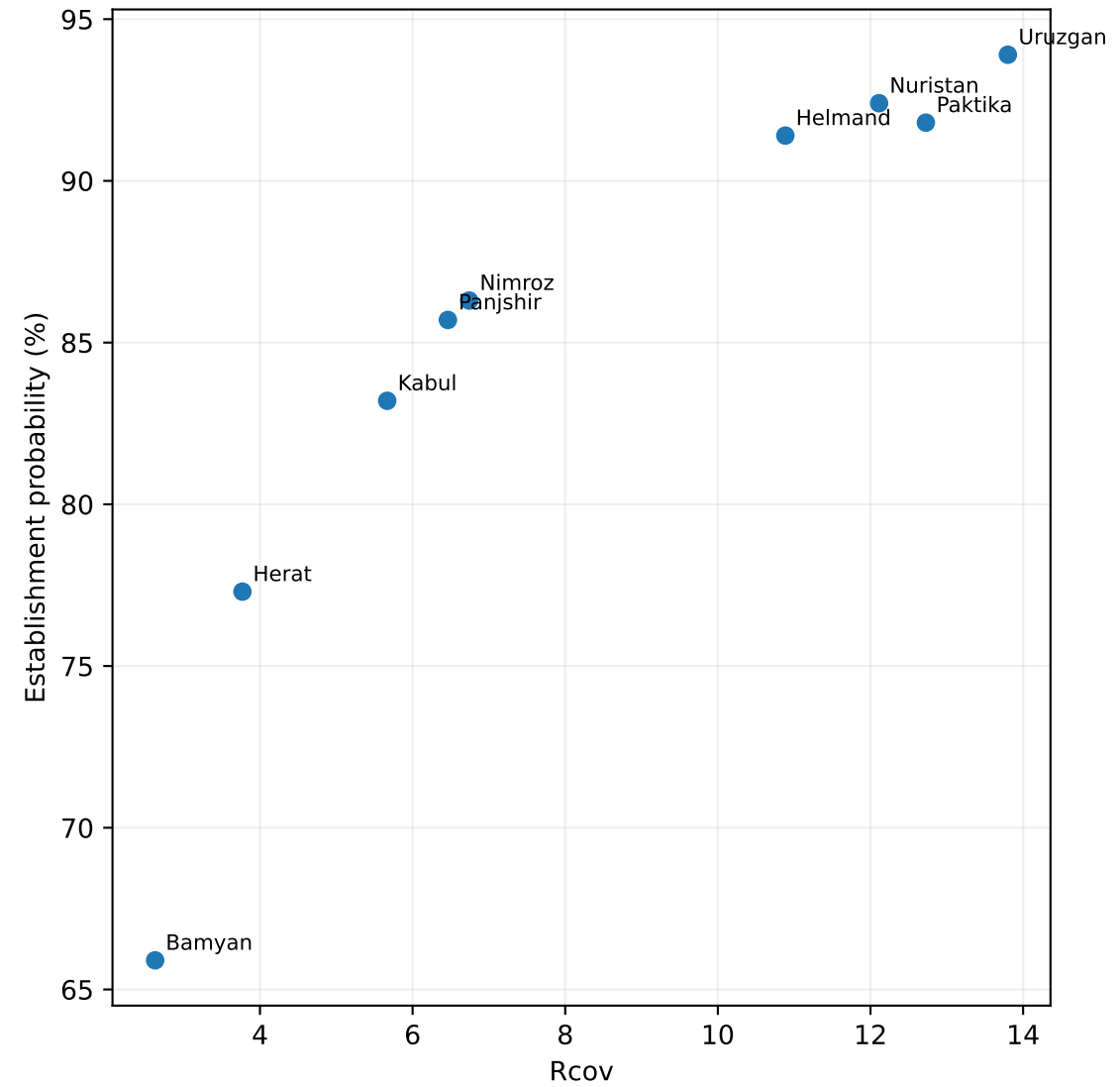
B. Rcov versus simulated establishment
