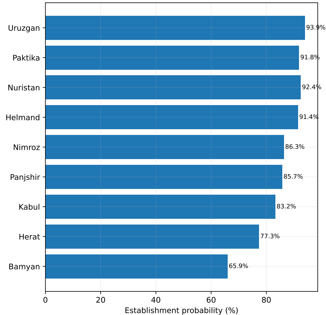
A. Single-importation establishment probability
