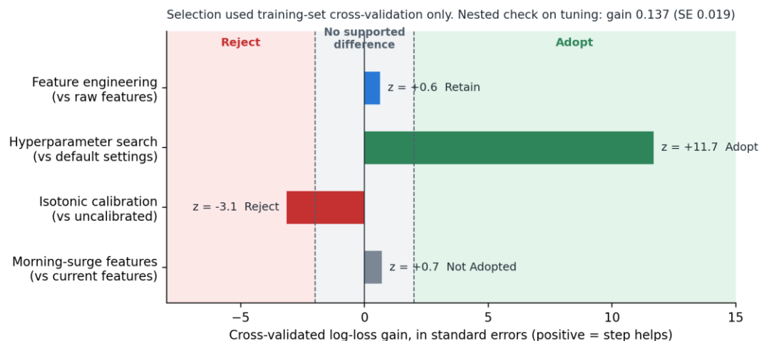
Figure 1. Cross-validated selection against the preset rule (training set only).
