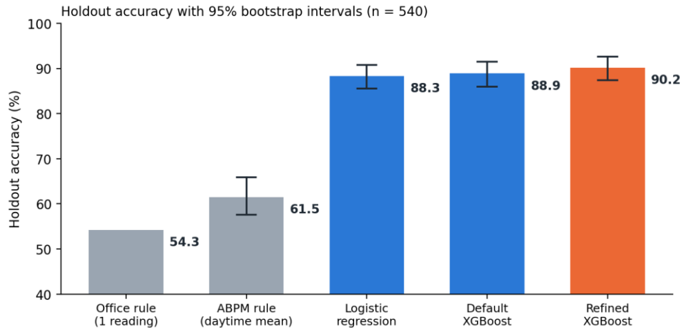
Figure 2. Holdout accuracy with 95% bootstrap intervals.
