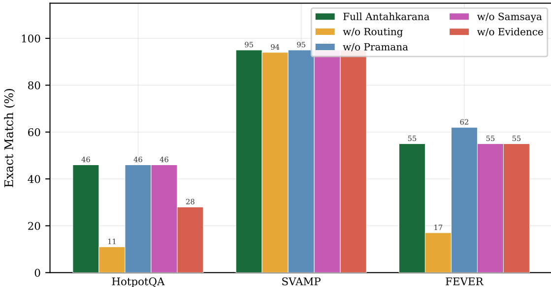
(f) Ablation Study — Exact Match
