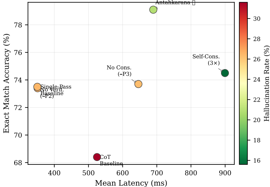
(f) Accuracy vs. Latency Trade-off
