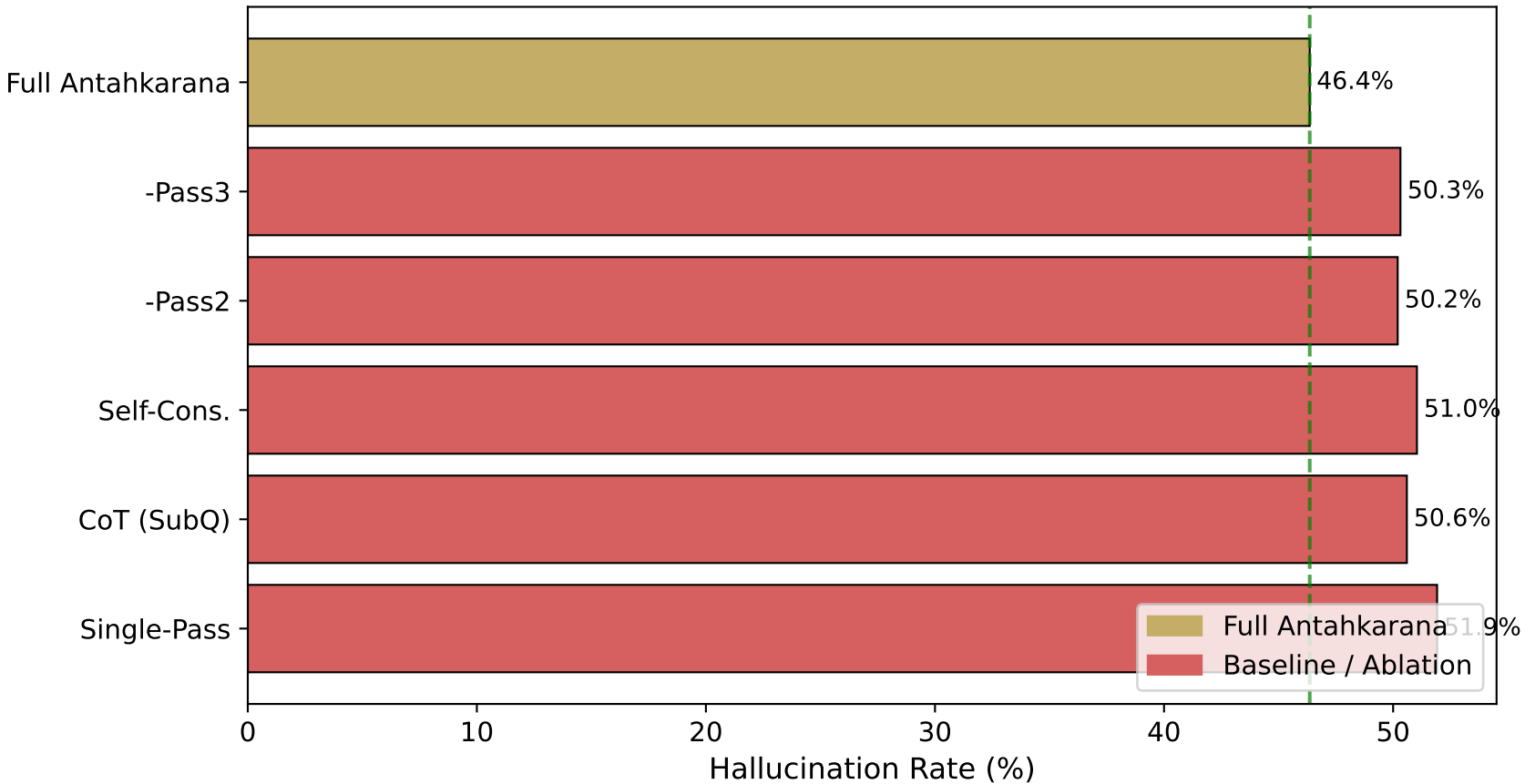
Figure 5: Hallucination Rate by Condition
