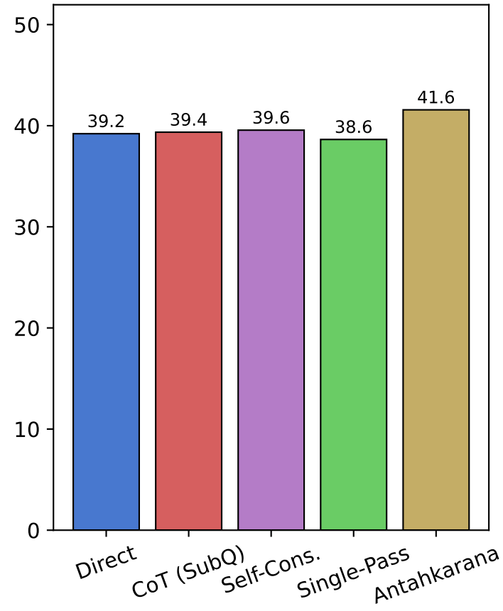
VQA Soft Accuracy (%)
