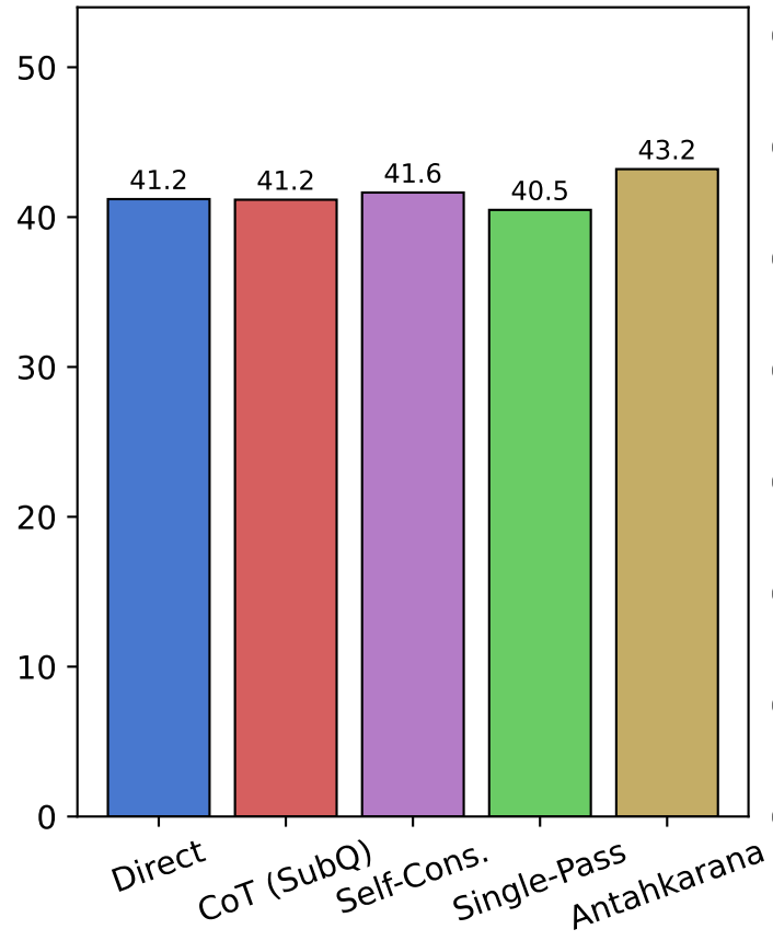
Exact Match (%)
