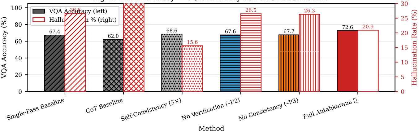
Fig. 1: Ablation Study — VQA Accuracy and Hallucination Rate
