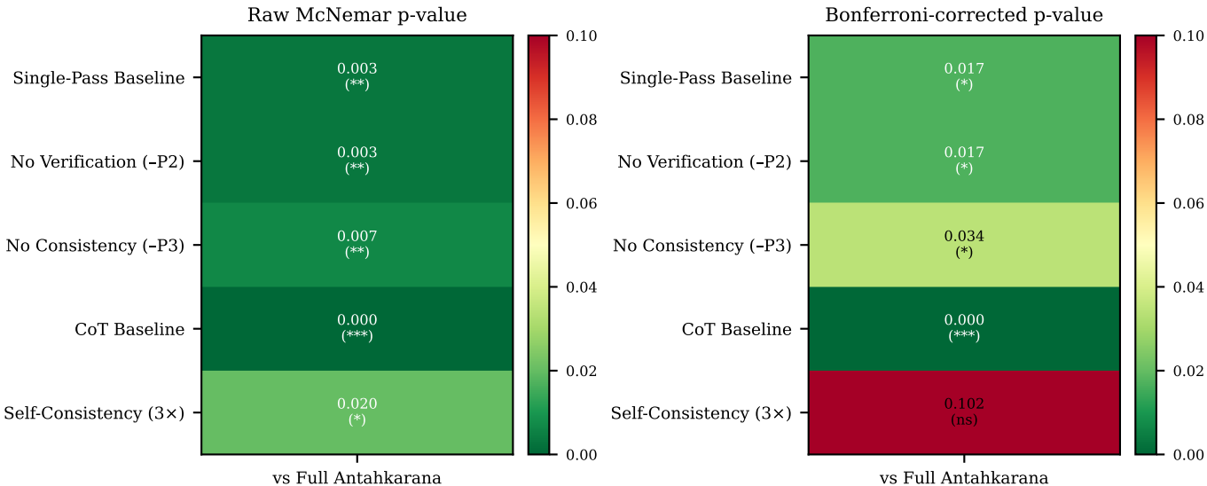
Fig. 5: Statistical Significance (McNemar \chi^2 )
