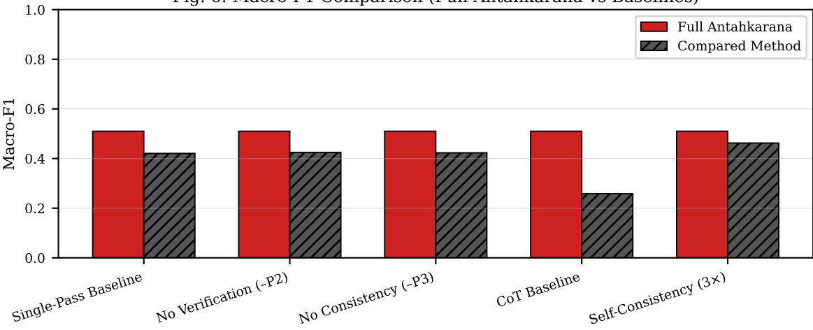
Fig. 6: Macro-F1 Comparison (Full Antahkarana vs Baselines)
