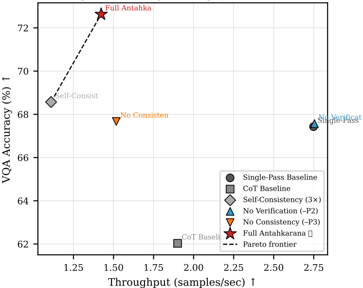
Fig. 7: Accuracy-Throughput Trade-off
