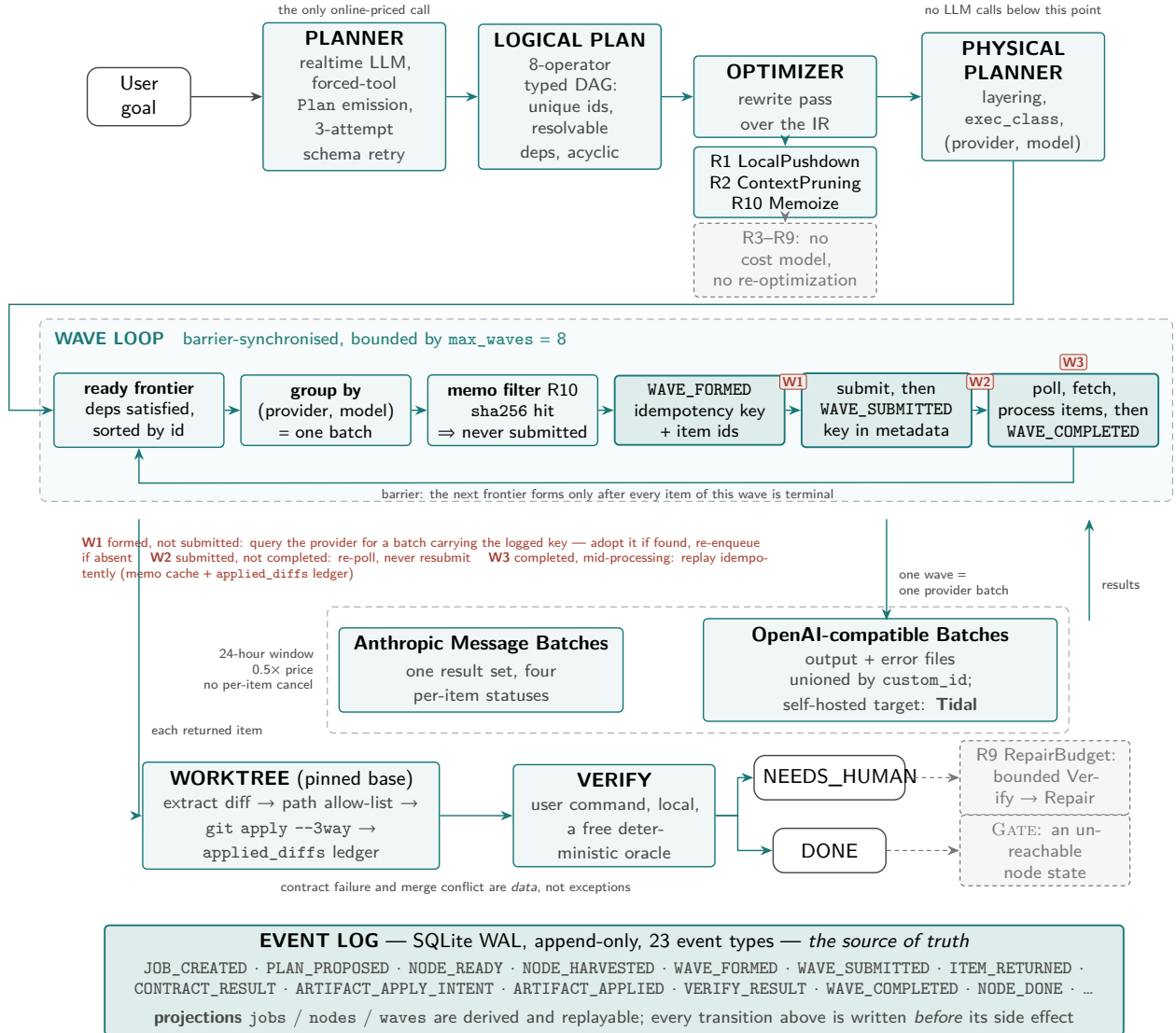
Figure 2: The LazyCode pipeline. Solid/accnt components are shipped code; dimmed components are designed with plumbing but not yet live (Section 7). The event log is the source of truth; jobs/nodes/waves tables are replayable projections. W1–W3 mark the three crash-safety windows of Section 4.4.
