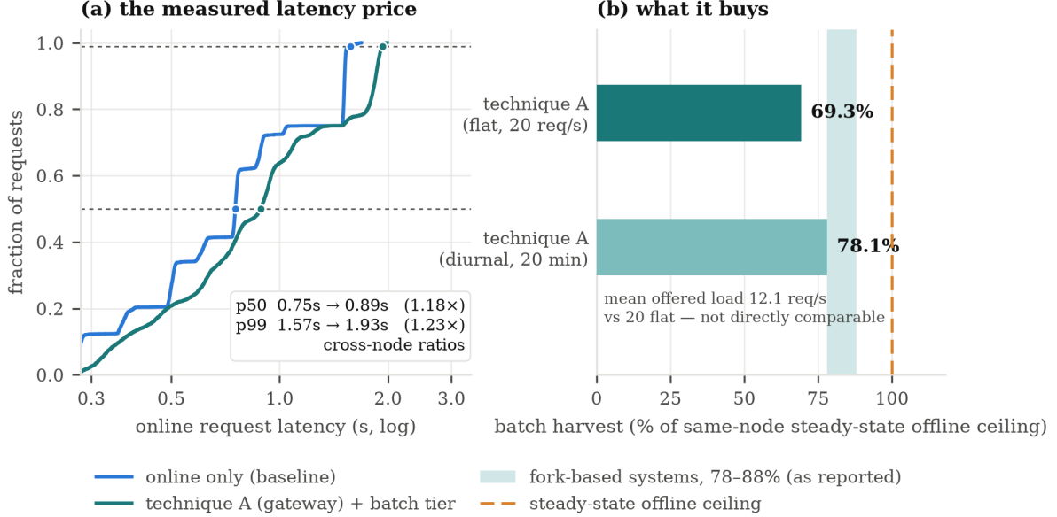
Figure 5: The headline trade at GPU scale. Left: online request-latency CDF, baseline versus technique A (cross-node). Right: batch harvest as a fraction of the node’s steady-state offline ceiling, with the band the fork-based literature reports shaded for reference.
