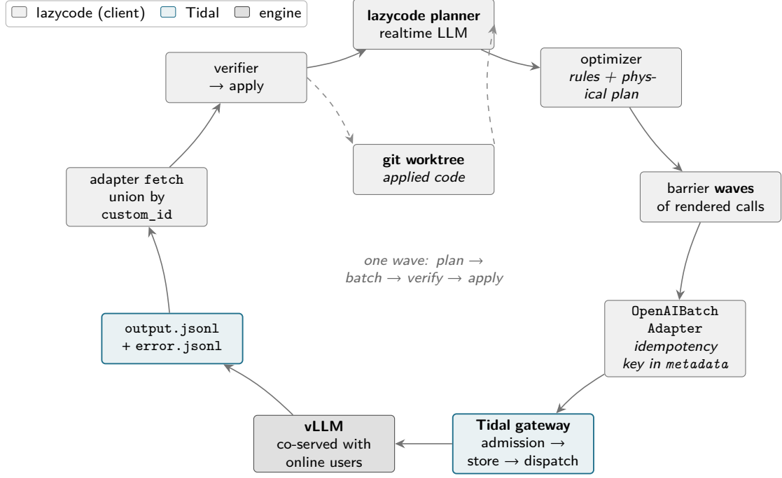
Figure 11: The complete loop. A realtime model plans the work; the optimizer lowers the plan into barrier waves of rendered calls; the OpenAIBatchAdapter uploads a wave as JSONL and stamps a server-side idempotency key in the batch’s metadata, so a crashed run can adopt its own orphaned batch. Tidal admits, stores and dispatches the wave into a vLLM that is simultaneously serving online users; the adapter fetches the output and error files and reassembles the wave by union over custom_id; the verifier runs the results and applies what passes into a git worktree, which feeds the next wave. This is the request lifecycle from client intent to applied code, entirely on self-hosted capacity at batch pricing. The client-side stages (planner, optimizer, waves, verifier) are detailed in the companion paper [29]; this figure shows only their interface to the serving tier.
