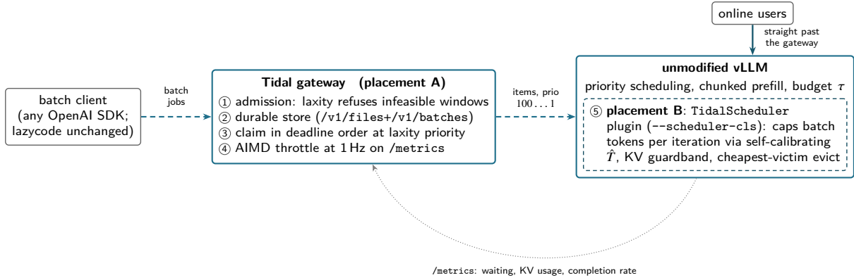
Figure 2: One policy, two placements. Batch jobs enter through an OpenAI-wire gateway that ① refuses infeasible windows at admission, ② stores jobs durably, ③ claims items in deadline order at their laxity priority, and ④ throttles dispatch by AIMD over the engine’s public metrics. Placement A stops there: the engine is stock vLLM, and online traffic never traverses the gateway. Placement B moves admission inside the engine ⑤ as a scheduler plugin that caps batch tokens per iteration against a self-calibrated latency model. Both are plugins; neither forks the engine.
