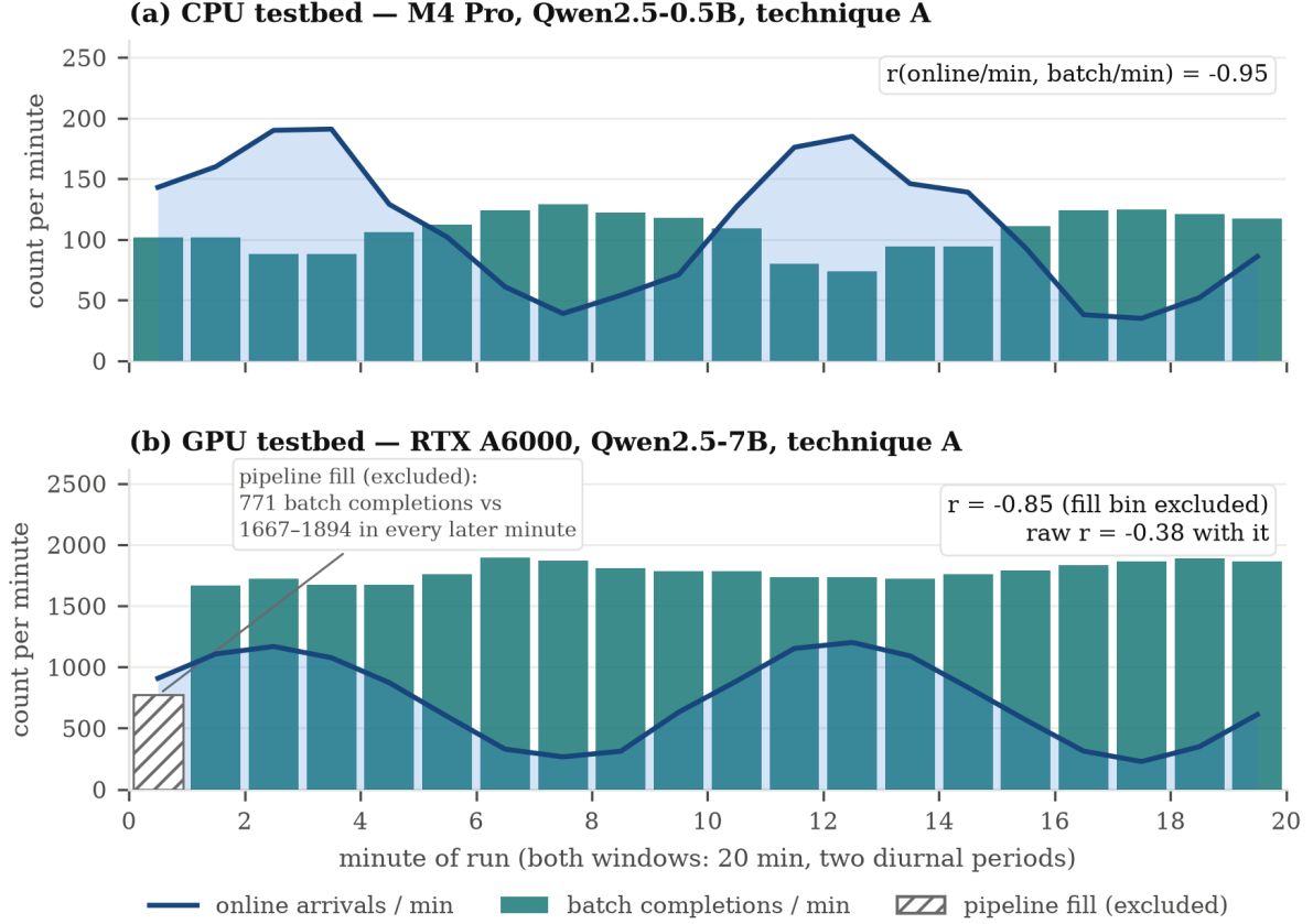
Figure 6: Batch fills the trough on both testbeds. Per-minute batch completions (bars) against online arrivals (line): CPU r = -0.95 (top), GPU r = -0.85 with the first-minute pipeline-fill bin shaded and excluded (bottom). On the CPU run the AIMD target never moved from its cap — the tide is produced entirely by engine-level priority scheduling, the two-level division of labor observed directly.
