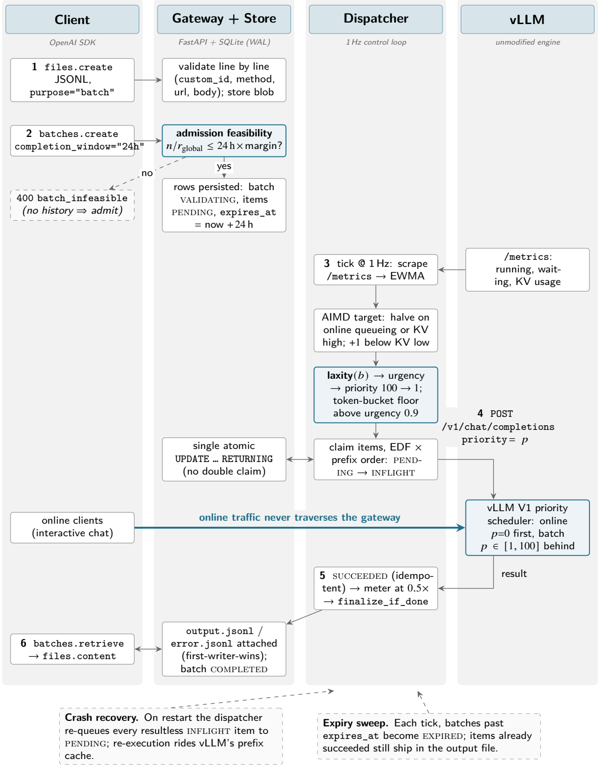
Figure 10: Technique A: the batch request lifecycle, end to end. A client uploads a JSONL file and creates a batch; the gateway validates every line and applies the laxity admission test, refusing with batch_infeasible any job whose projected completion exceeds the window times a margin, and otherwise persisting PENDING items with a 24-hour expires_at . A 1 Hz dispatcher scrapes the engine’s public metrics, sets an AIMD in-flight target, computes each batch’s laxity-derived priority, claims items in deadline × prefix order and submits them to vLLM as ordinary low-priority chat completions — while online clients (thick arrow) reach the engine directly, never through the gateway. Results settle idempotently, are metered at the batch discount, and are assembled into the output and error files the client downloads.
