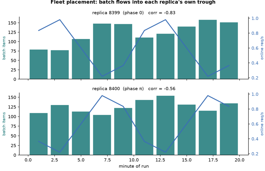
Figure 13: A-F mechanism, per replica: measured batch completions (bars) against each replica’s own analytic online rate (line). Volume splits evenly; timing follows each replica’s trough.
