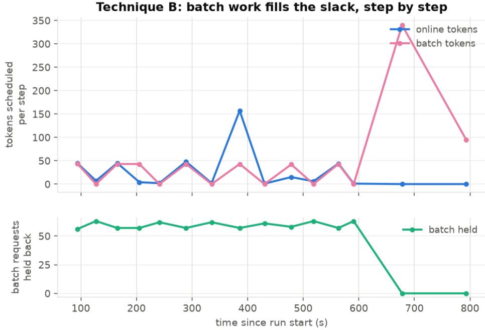
Figure 9: Technique B, step by step: online and batch tokens scheduled per iteration (top) and batch requests held back by the pre-gate (bottom). Online traffic stops near t = 600 s; the held set empties and batch takes the whole budget — offline mode.
