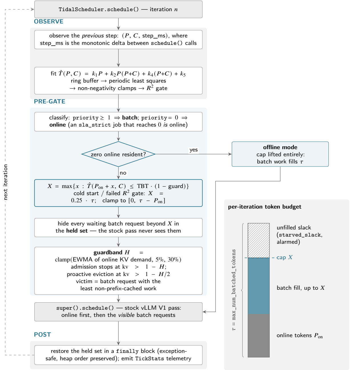
Figure 4: Technique B: one engine iteration. TidalScheduler wraps rather than reimplements the stock schedule() . Before the stock pass it feeds the previous step’s (P, C, \text{step\_ms}) to a continuously refitted latency model, solves that model for the largest batch-token cap X that keeps the step inside the guarded inter-token budget, and hides every waiting batch request beyond X — lifting the cap entirely when no online request is resident. A KV guardband stops batch admission before online bursts can be starved of blocks and evicts the cheapest batch victim under further growth. After the stock pass the held set is restored in a finally block. The side panel shows what X governs: online tokens occupy the bottom of the \tau -token budget, batch work fills up to the cap, and whatever is left unfilled is reported as starved slack.
