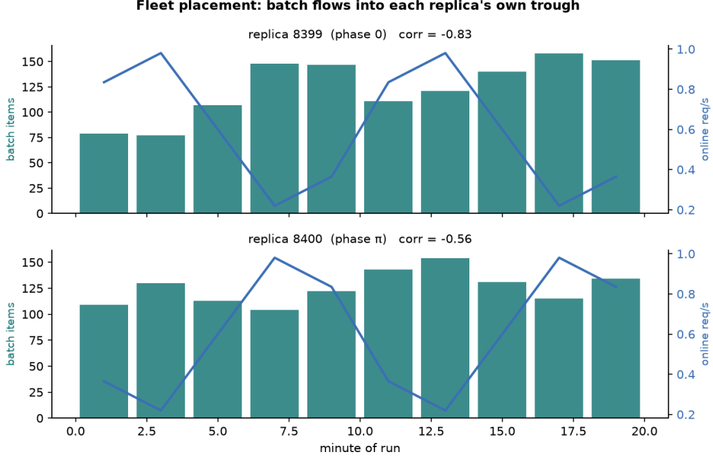
Figure 13: A-F mechanism, per replica. Measured batch completions (bars) against each replica’s own analytic online arrival rate (line; the seeded diurnal schedules, phases 0 and \pi ). Batch volume splits almost evenly across the replicas (1239 / 1255) but is timed into each replica’s trough — correlation -0.83 and -0.56 . Raw data: results/fleet_a.json in the repository.
