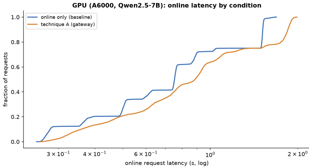
Figure 9: GPU online request latency, baseline versus technique A (A6000, Qwen2.5-7B, 20 req/s Poisson). The co-location tax that cost 2.54\times p50 on the CPU testbed is 1.18\times here — a cross-node comparison: the two arms ran on different (but \pm 0.62\% -matched) A6000 nodes.
