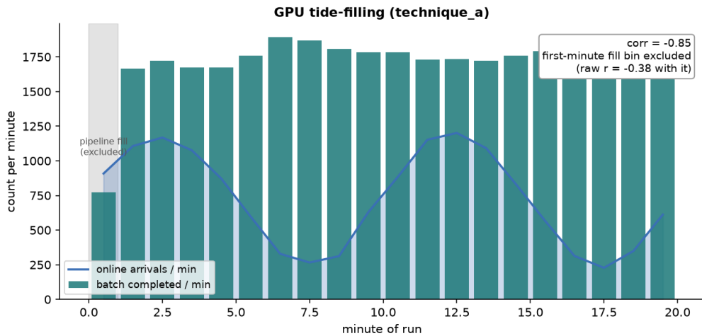
Figure 11: GPU tide-filling under a sinusoidal online load (technique A, 20-minute window, peak 20 req/s). Per-minute batch completions anti-correlate with online arrivals at r = -0.85 once the first-minute pipeline-fill bin (shaded) is excluded; including that bin gives -0.38 , which is a startup artifact rather than a weak tide.
