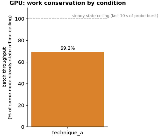
Figure 10: Batch output throughput recovered while online traffic is served, as a fraction of the same node’s independently probed steady-state dedicated-offline ceiling (last 10 s of the probe burst): 69.3% under flat load, 78.1% under diurnal load.
