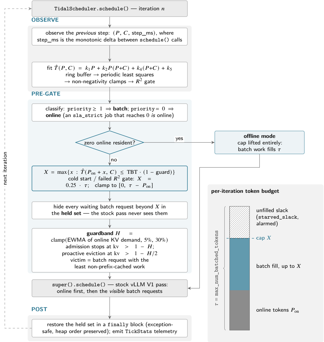
Figure 3: Technique B: one engine iteration. TidalScheduler wraps rather than reimplements the stock schedule(). Before the stock pass it feeds the previous step’s (P, C, \text{step\_ms}) to a continuously refitted latency model, solves that model for the largest batch-token cap X that keeps the step inside the guarded inter-token budget, and hides every waiting batch request beyond X — lifting the cap entirely when no online request is resident. A KV guardband stops batch admission before online bursts can be starved of blocks and evicts the cheapest batch victim under further growth. After the stock pass the held set is restored in a finally block. The side panel shows what X governs: online tokens occupy the bottom of the \tau -token budget, batch work fills up to the cap, and whatever is left unfilled is reported as starved slack.
