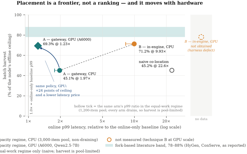
Figure 8: Placement is a frontier, not a ranking. Online p99 ratio (log) against harvest, all measured arms, with the band the fork-based literature reports shaded. The same policy moves from the CPU point to the GPU point when the binding resource changes; technique B's GPU point was not obtained (open marker).
