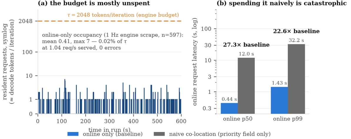
Figure 1: The budget is mostly unspent — and spending it naively is catastrophic. Left: resident online requests ( \approx decode tokens per iteration) under online-only traffic on our testbed — mean 0.41, i.e. 0.02% of the \tau = 2048 budget. Right: the online latency price of naive co-location (vLLM’s priority field alone), 27.3×/22.6× p50/p99 (Section 5.4) — admission priority does not bound resident-request contention, which is why something must meter how much batch work exists at all.
