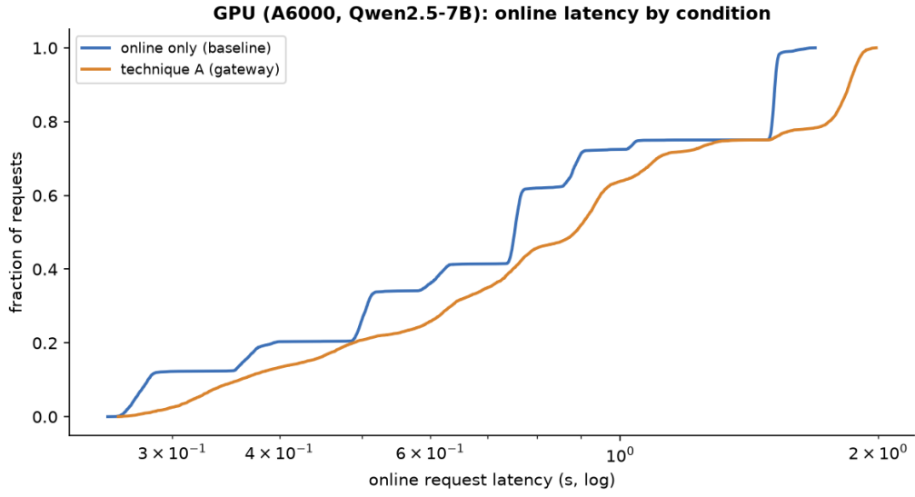
Figure 9: GPU online request latency, baseline versus technique A (A6000, Qwen2.5-7B, 20 req/s Poisson). The co-location tax that cost 2.54\times p50 on the CPU testbed is 1.18\times here.
