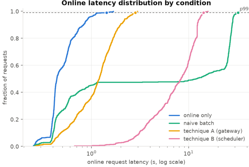
Figure 5: Measured distribution of online request latency under each condition. Reporting the full CDF rather than the tail alone is deliberate: the medians degrade more than the tails everywhere.
