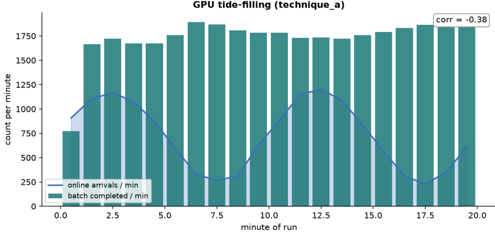
Figure 11: GPU tide-filling under a sinusoidal online load (technique A, 20-minute window, peak 20 req/s). Anti-correlation is only r = -0.38 because batch runs near the node ceiling in both tides — the head-room is so large that the trough is barely a constraint.
