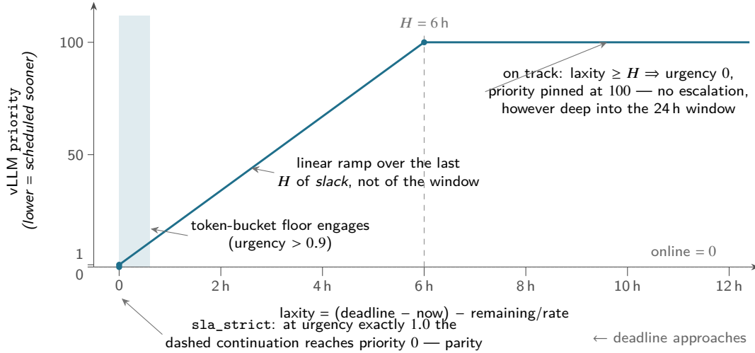
Figure 1: The escalation curve. Priority is flat at the lowest band (100) for every job with at least a full escalation horizon H = 6 h of slack, then ramps linearly to 1 — one notch below online — as laxity runs out. Scaling urgency by H rather than by the 24-hour window is what keeps a healthy job from escalating on the clock alone. Above urgency 0.9 (shaded) a token bucket guarantees a minimum admission rate, and the sla_strict dial allows the dashed continuation to priority 0 at urgency exactly 1.0.
