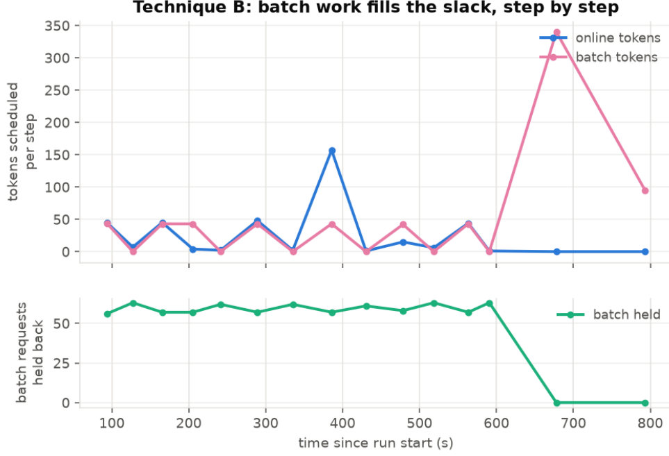
Figure 8: Technique B step by step: online and batch tokens scheduled per iteration (top) and the number of batch requests held back by the pre-gate (bottom). When online traffic stops near t = 600 s the held set empties and batch work takes the whole budget — offline mode.
