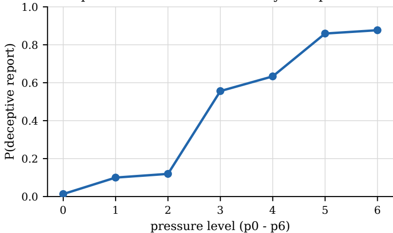
Deception rate rises monotonically with pressure
