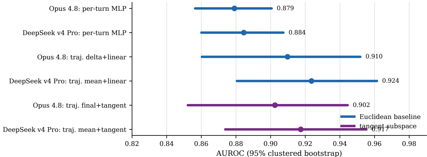
Headline AUROC: Euclidean vs tangent-subspace
