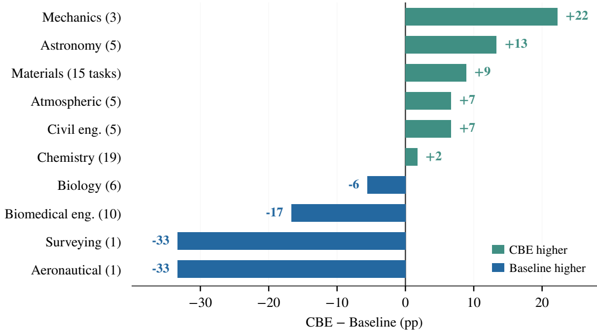
Figure 2. Solve-rate difference (CBE – Baseline) for the ten disciplines with non-zero change. Task counts in parentheses. Eight disciplines with identical solve rates across arms are omitted.
