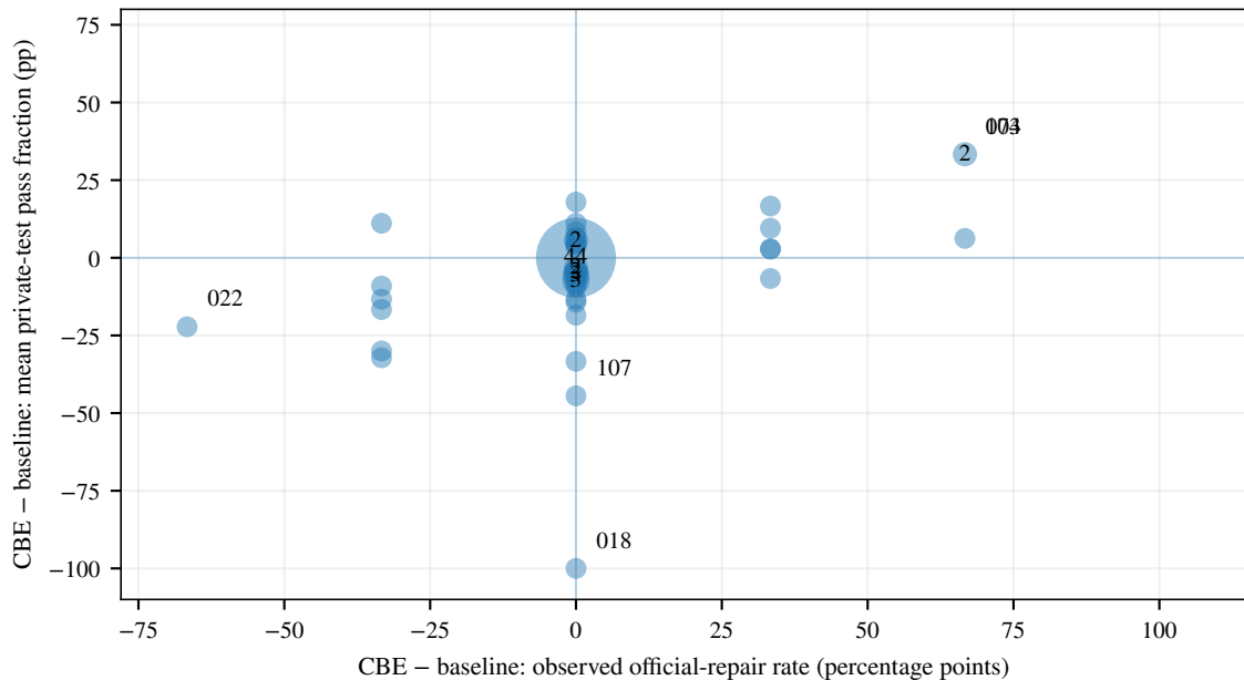
Exact ties can hide changes in partial test coverage
