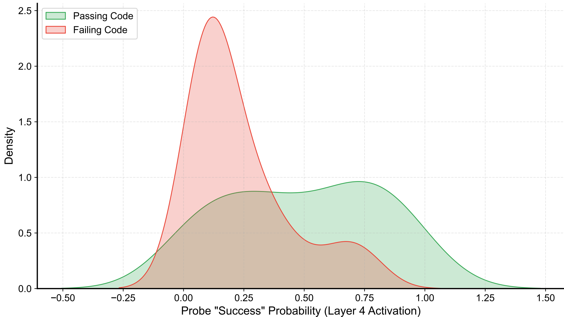
Probe Confidence vs. Execution Success
