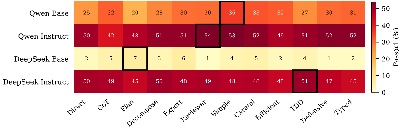
Per-style Pass@1 averaged over HumanEval + MBPP (best style boxed per model)
