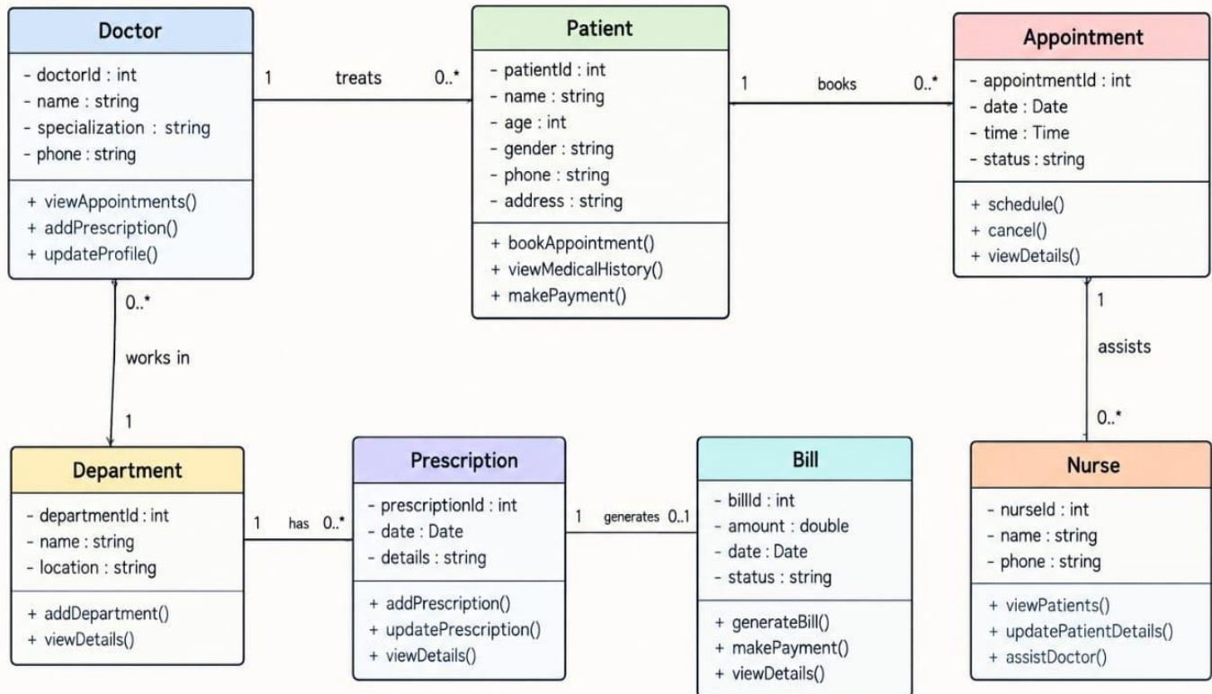
Hospital Management System – Class Diagram
