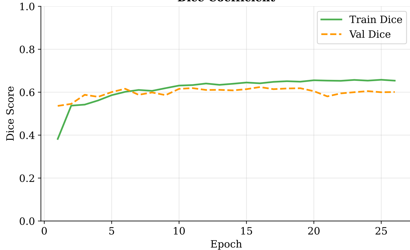
Dice Coefficient
