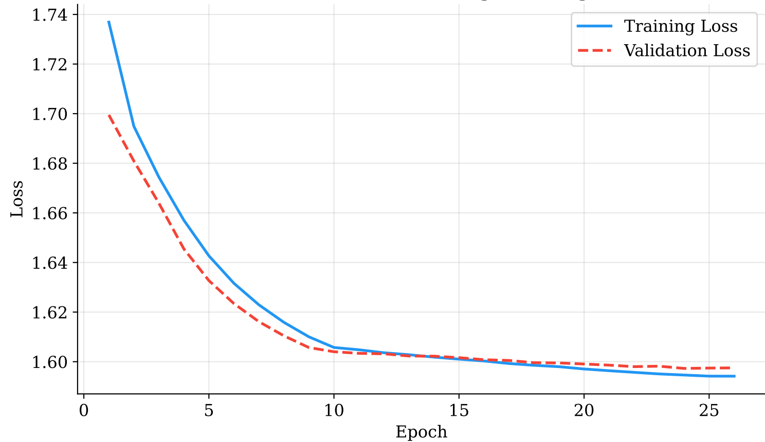
Dice-BCE Loss During Training
