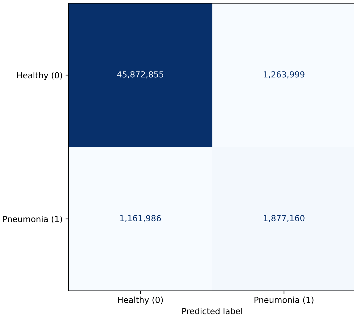
Pixel-Level Confusion Matrix MobileNetV2-UNet on RSNA Test Set
