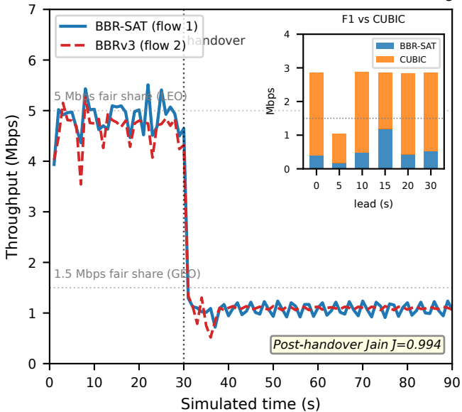
(a) F1: Shared LEO→GEO handover (lead=0, 2-run avg)
