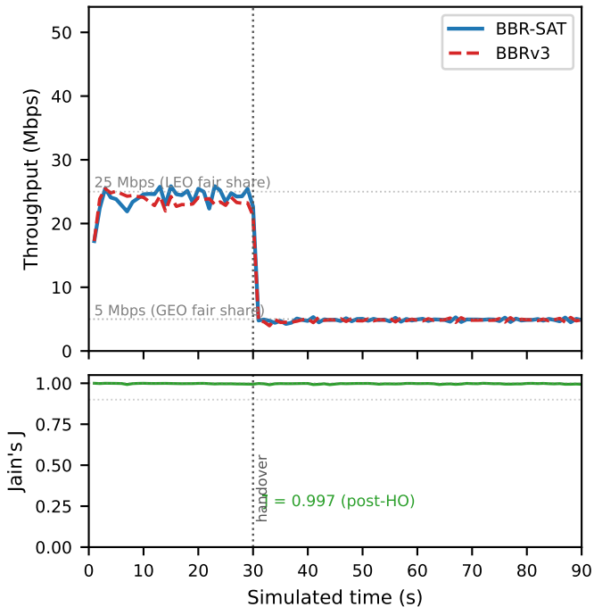
F1: BBR-SAT vs BBRv3 — shared LEO→GEO handover (lead=0)
