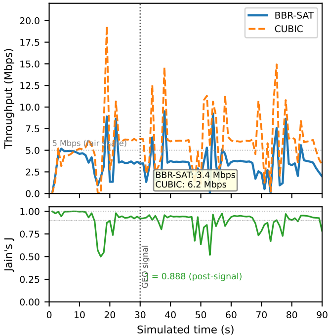
F3: BBR-SAT vs CUBIC — steady-state GEO (2-run avg)
