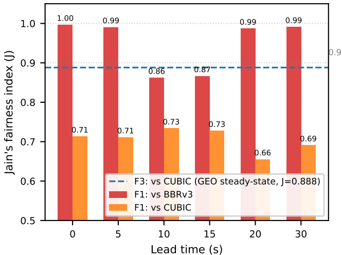
Jain's J vs lead time — Experiment 2
