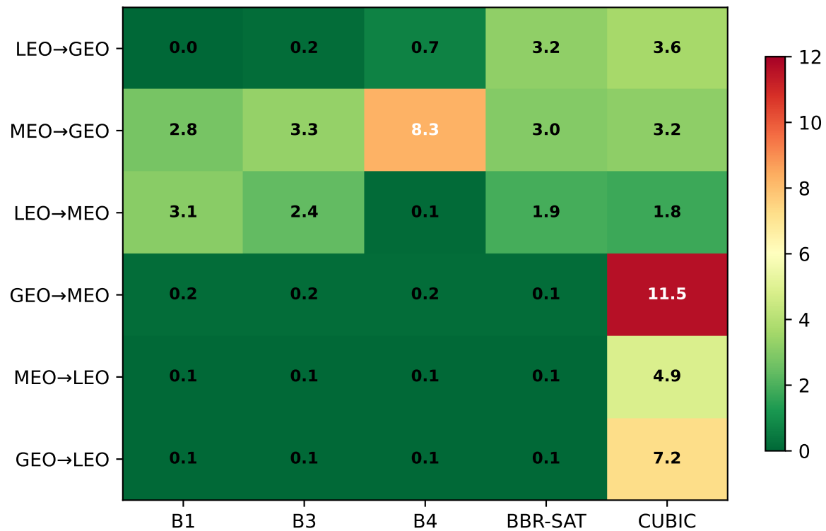
(b) Steady-state throughput std dev (Mbps) Red=unstable, Green=stable
