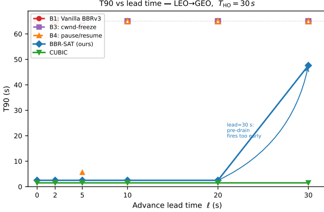
Fig. 1. T90 vs. advance lead time for the LEO→GEO transition ( T_{HO} = 30 s, no loss). BBR-SAT maintains a flat 2.5 s across \ell \in [0, 20] s; open markers at the top dashed line denote non-convergent (N/C) trials.
