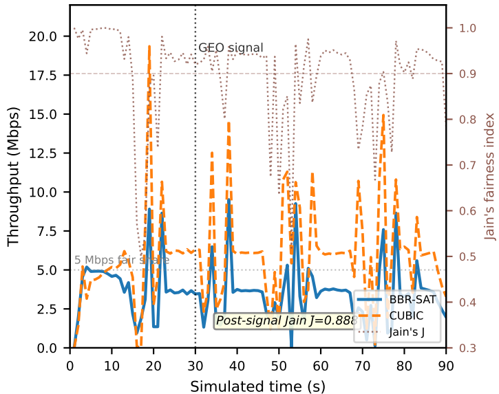
(b) F3: BBR-SAT vs CUBIC — steady-state GEO (2-run avg)
